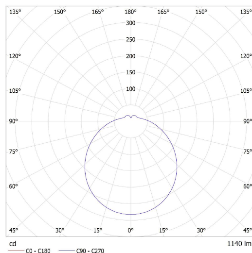
Lucis S26.L14.CA2 CHARON PMMA LED / LDC (Polar)
